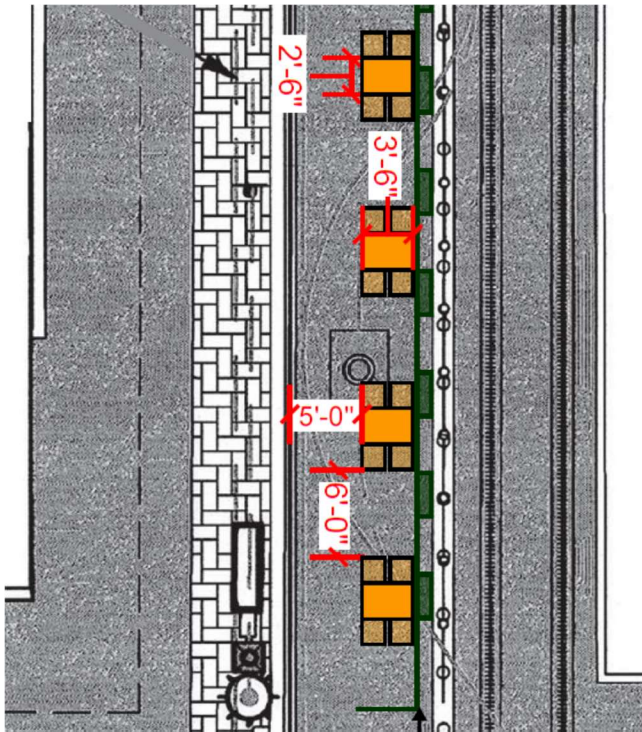
Furniture Plan typical layout with dimensional requirements
